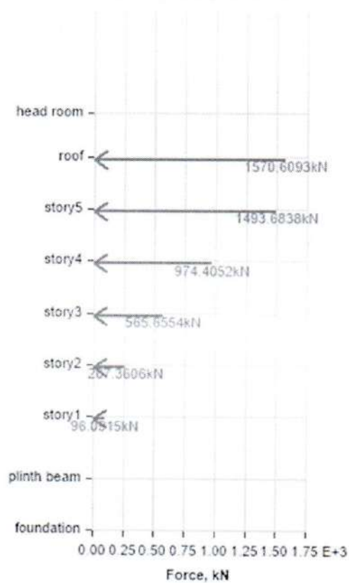
Lateral Load to Stories - Y
