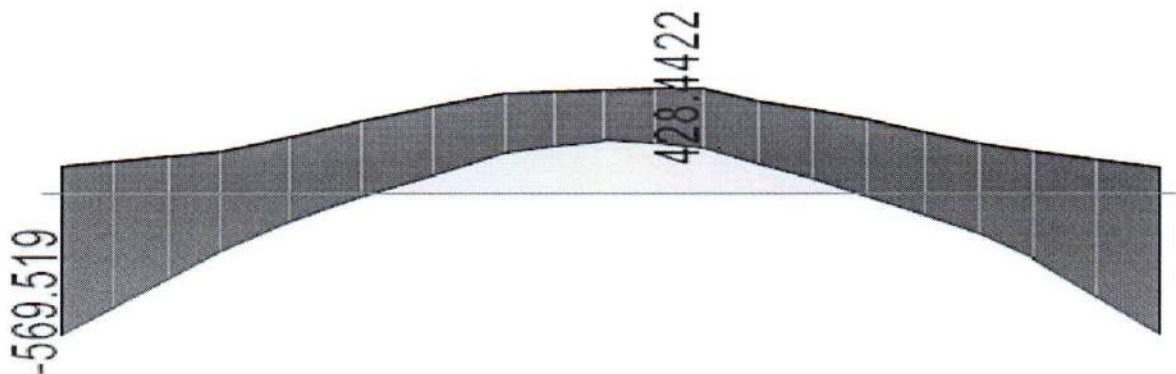
Critical Bending Moment Diagram
