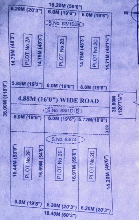
PROPOSED SUB-DIVISION PLAN (Scale 1:200)
