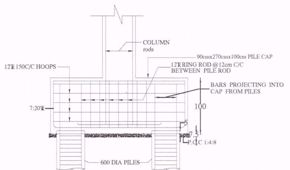
PILE CAP DETAIL - P8
