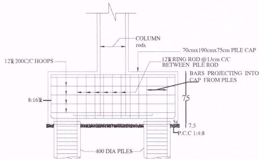
PILE CAP DETAIL-P5
