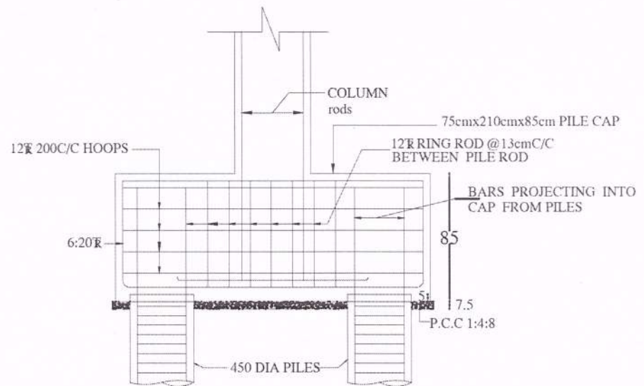
PILE CAP DETAIL - P6
