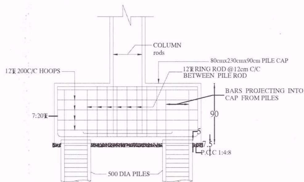
PILE CAP DETAIL - P7
