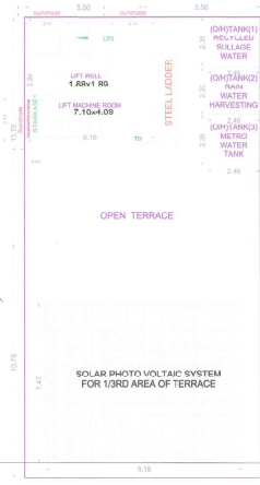
TERRACE FLOOR PLAN (PROPOSED)
