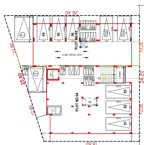
SITE CUM STILT FLOOR PLAN
