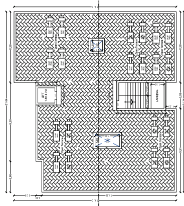
HEAD ROOM / TERRACE FLOOR PLAN
