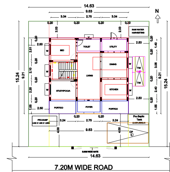
SITE CUM GROUND FLOOR PLAN (PROPOSED)
