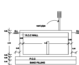
SECTION ON D-4
