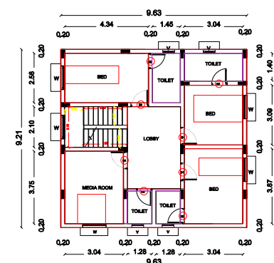
FIRST FLOOR PLAN (PROPOSED)
