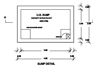
SUMP DETAIL
