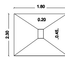
COLUMN PLAN
