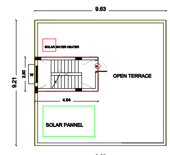
TERRACE FLOOR PLAN (PROPOSED)
