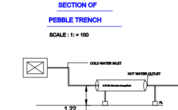
SOLAR WATER HEATING SYSTEM DETAILS
