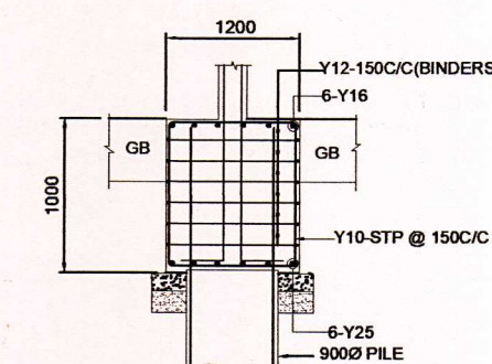
SECTION - 7-7
