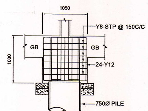
SECTION - 1-1
