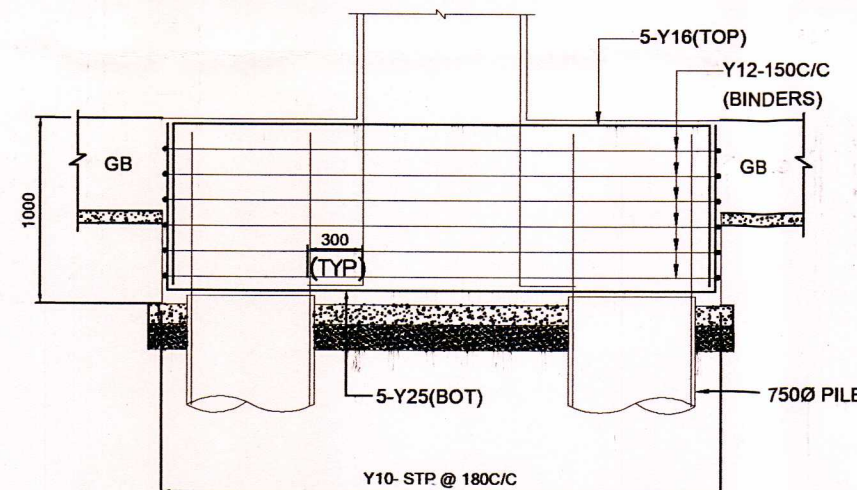
SECTION - 3-3
