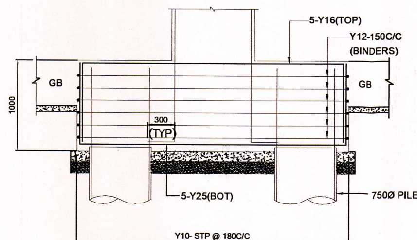
SECTION - 5-5
