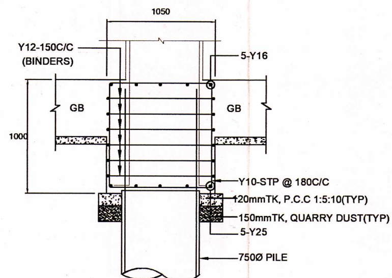
SECTION - 4-4
