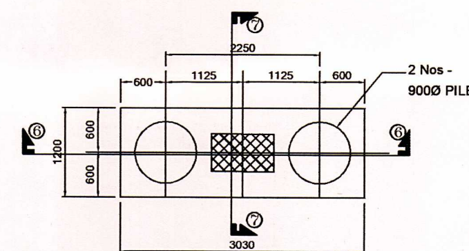
PILE-P3
