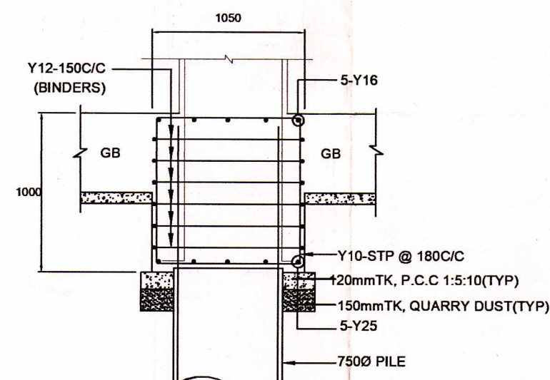
SECTION - 2-2
