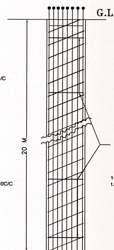
TYPICAL SECTION OF PILE BORED CAST IN-SITU PILE
