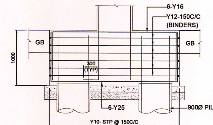
SECTION - 6-6
