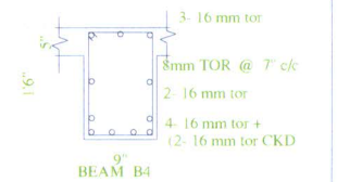
BEAM B4
