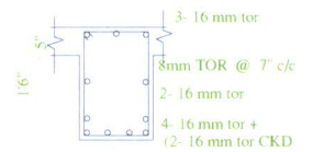
BEAM B4
