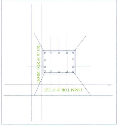
COLUMN SECTION
