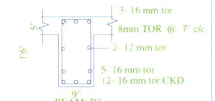
BEAM B3
