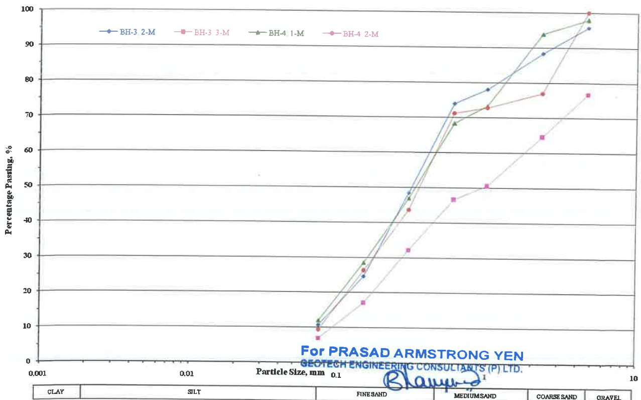
Grain Size Distribution Curves Boring 3 & 4
