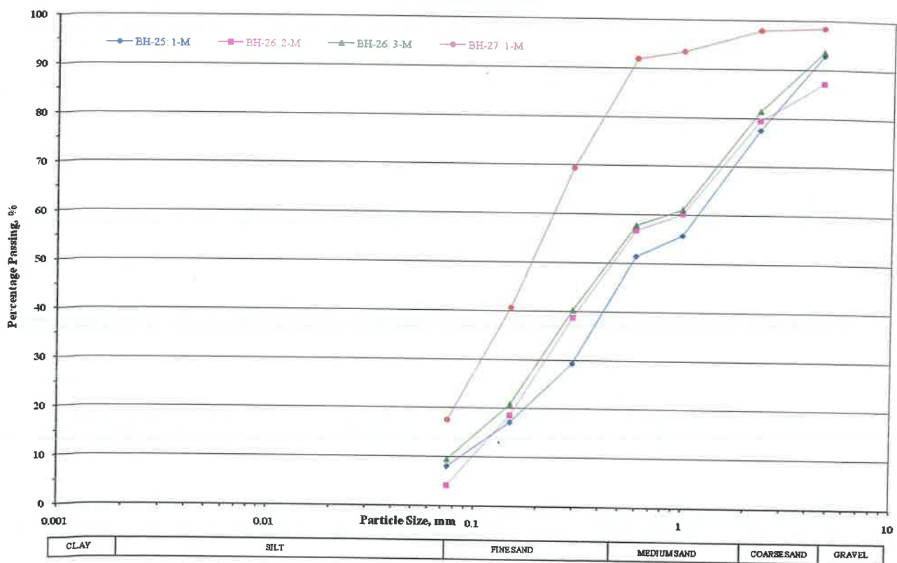
Grain Size Distribution Curves Boring 25, 26 & 27
