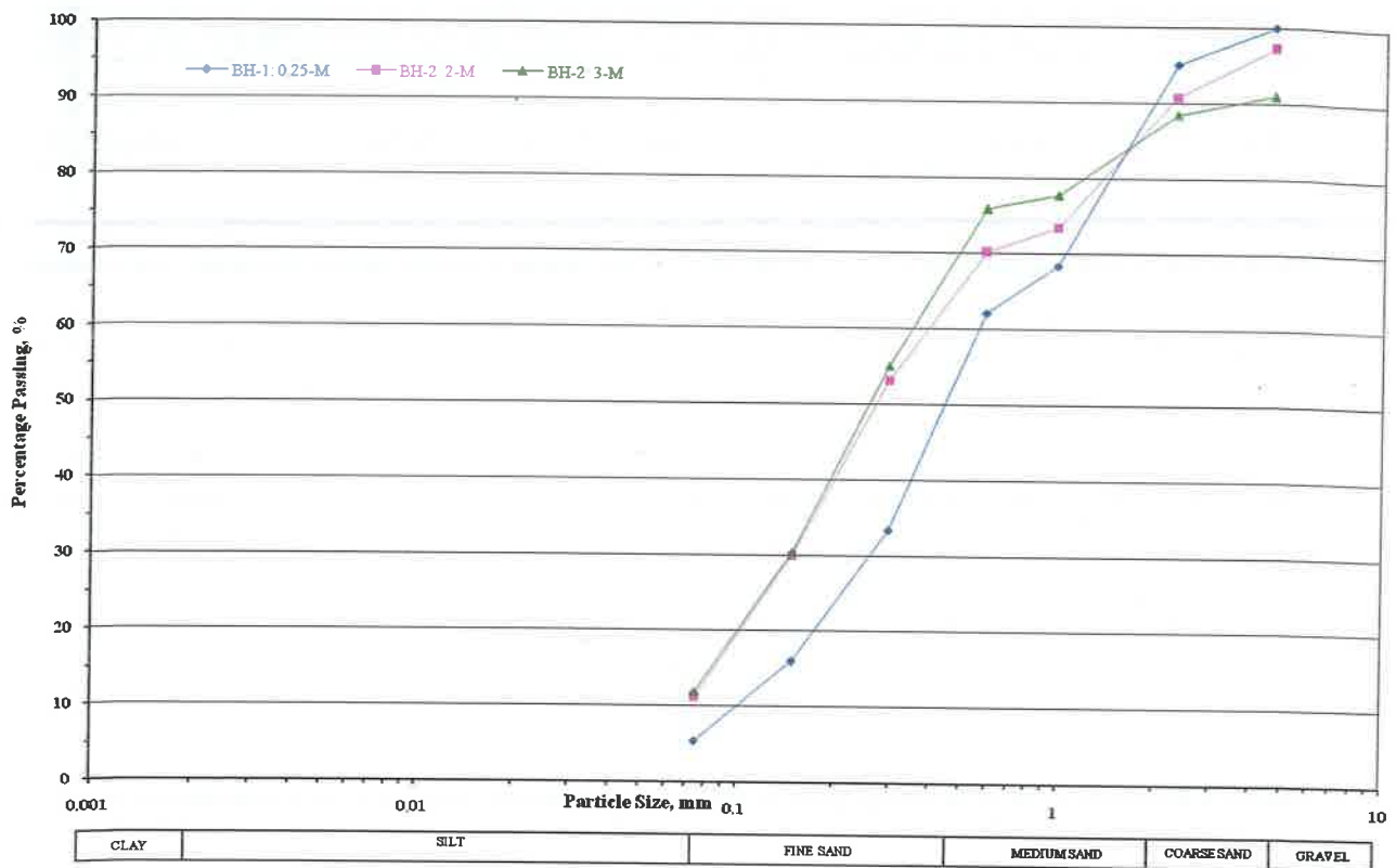
Grain Size Distribution Curves Boring 1 & 2
