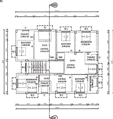
PRO.. FIRST & SECOND FLOOR PLAN
