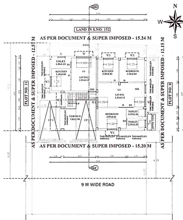
SITE CUM PRO.. GROUND FLOOR PLAN
