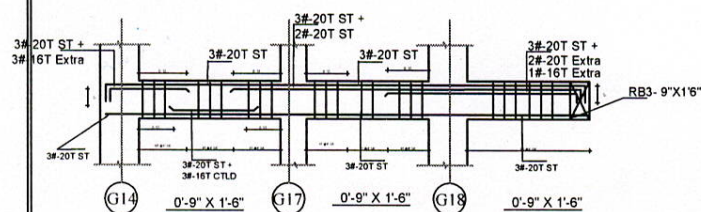
LONGITUDINAL SECTION OF GRID - G14 TO G18
