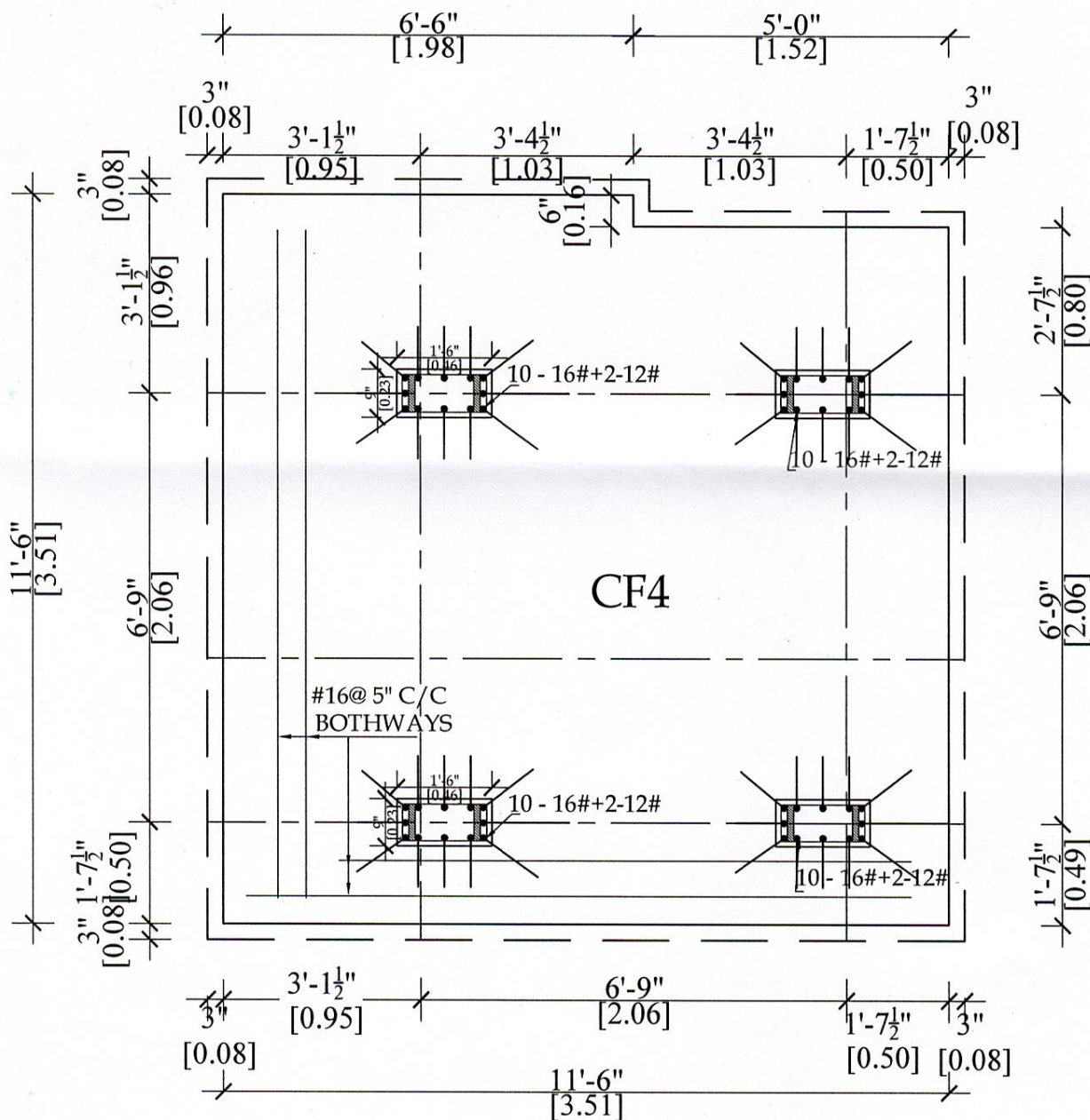
SECTION
