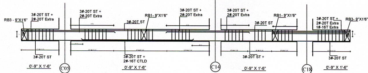
LONGITUDINAL SECTION OF GRID - C05 TO C18
