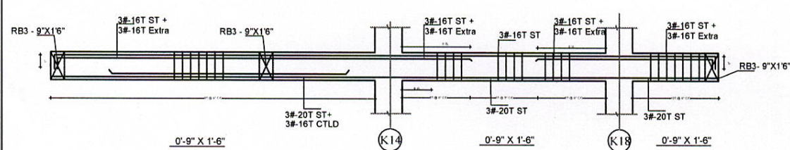
LONGITUDINAL SECTION OF GRID - K14 TO K18
