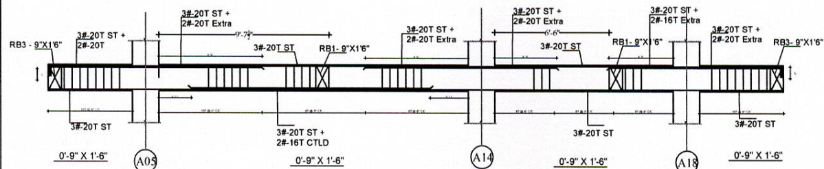
LONGITUDINAL SECTION OF GRID - A05 TO A18
