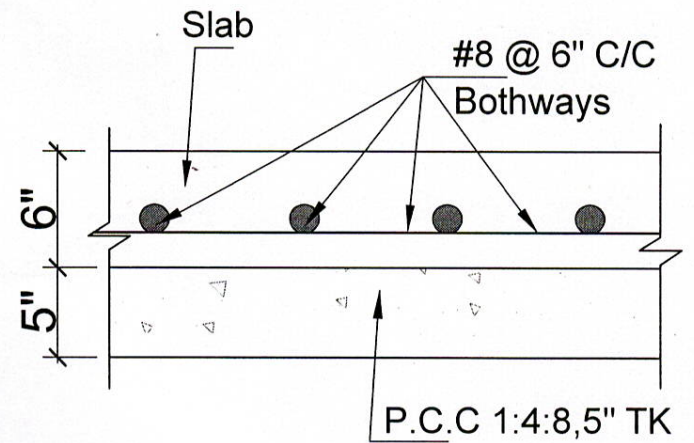
FLOORING SLAB DETAILS
