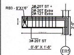
LONGITUDINAL SECTION OF GRID - E05
