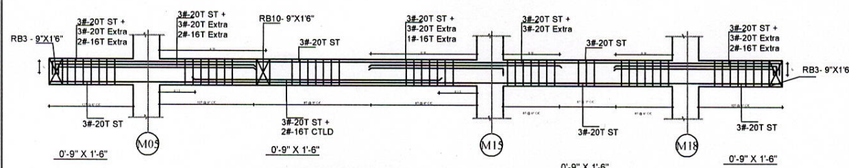
LONGITUDINAL SECTION OF GRID - M05 TO M18
