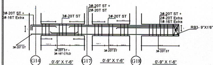
LONGITUDINAL SECTION OF GRID - G14 TO G18
