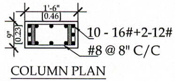
COLUMN PLAN
