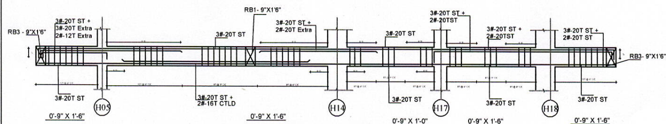
LONGITUDINAL SECTION OF GRID - H05 TO H18
