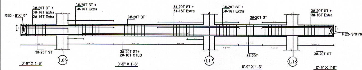
LONGITUDINAL SECTION OF GRID - L05 TO L18
