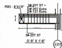
LONGITUDINAL SECTION OF GRID - E05
