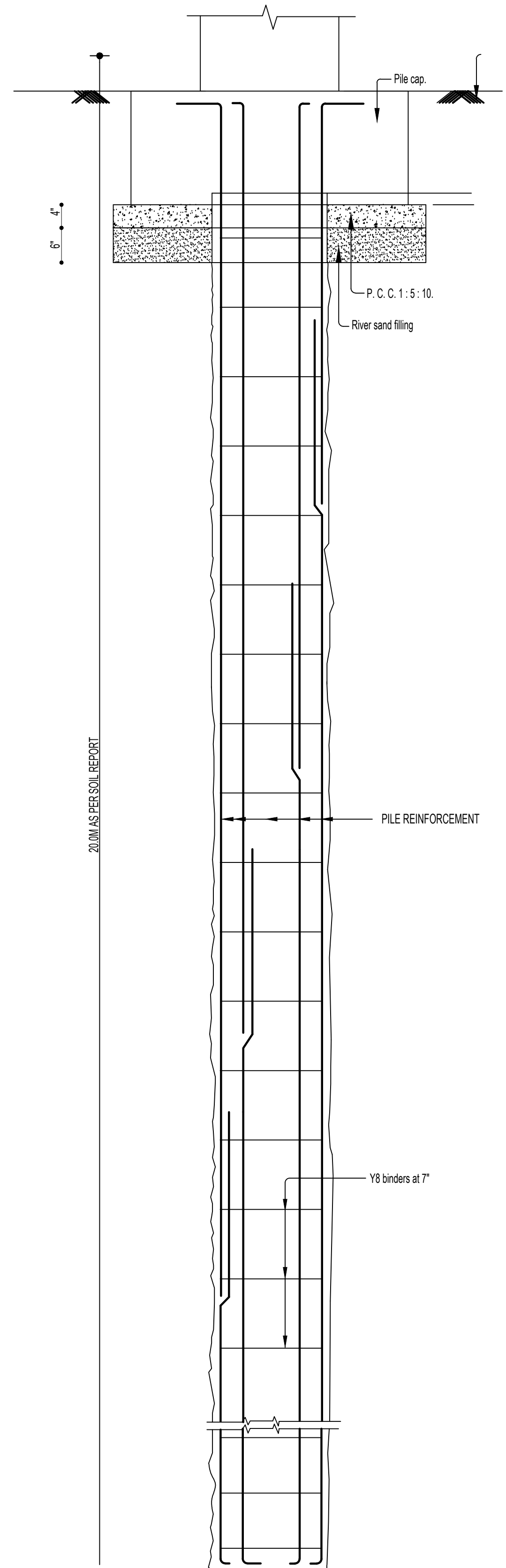
LONGITUDINAL SECTION OF BORED CAST-IN-SITU PILES
