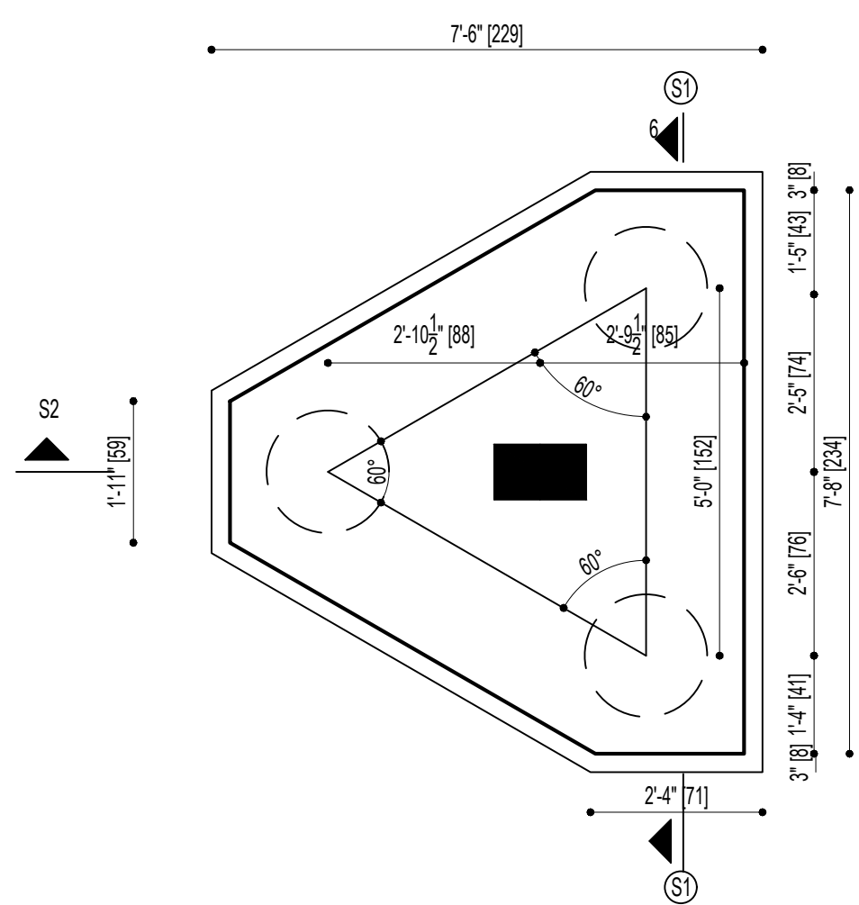
PLAN OF PILE CAP
