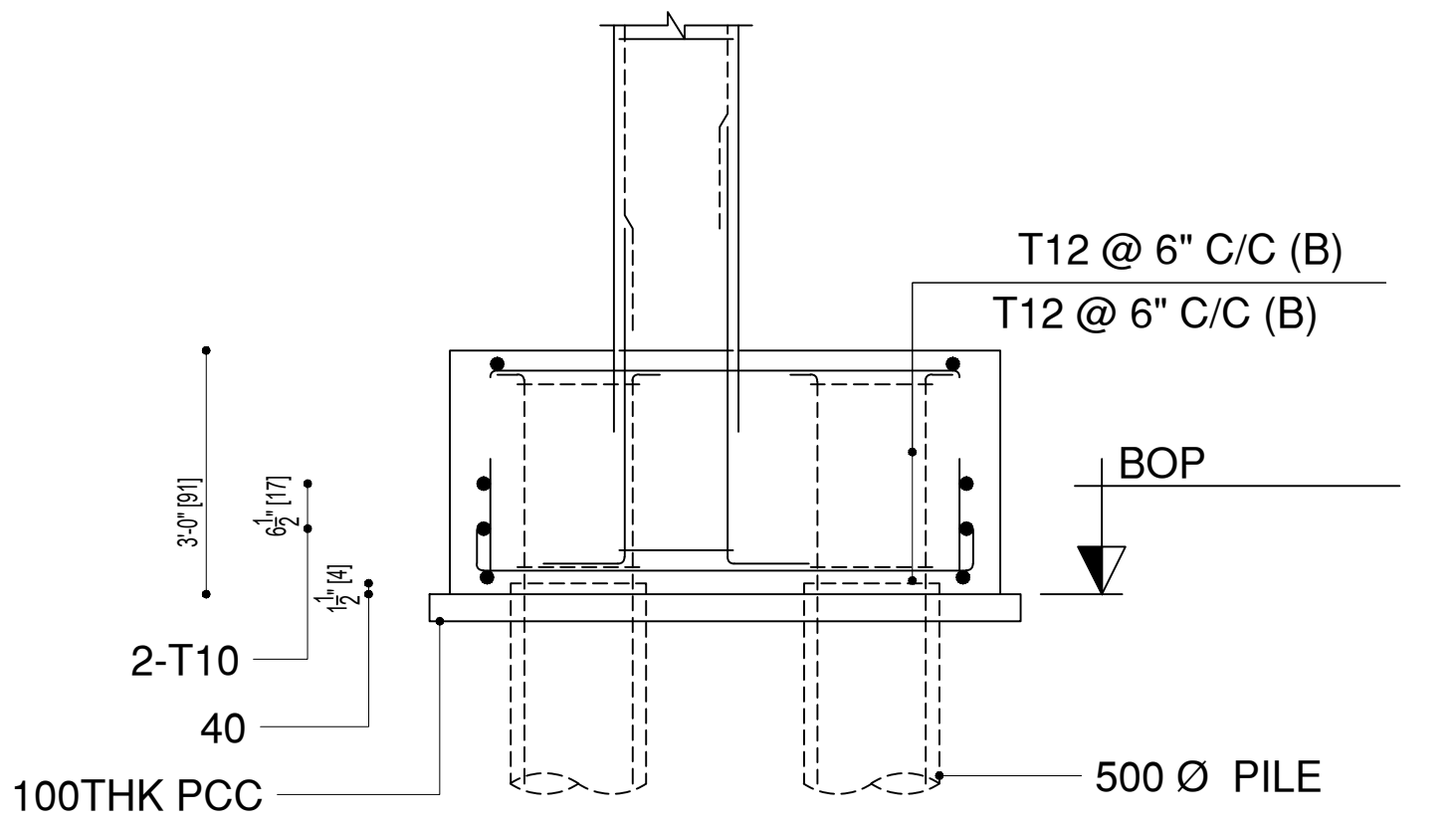
SECTION - S2 - S2
