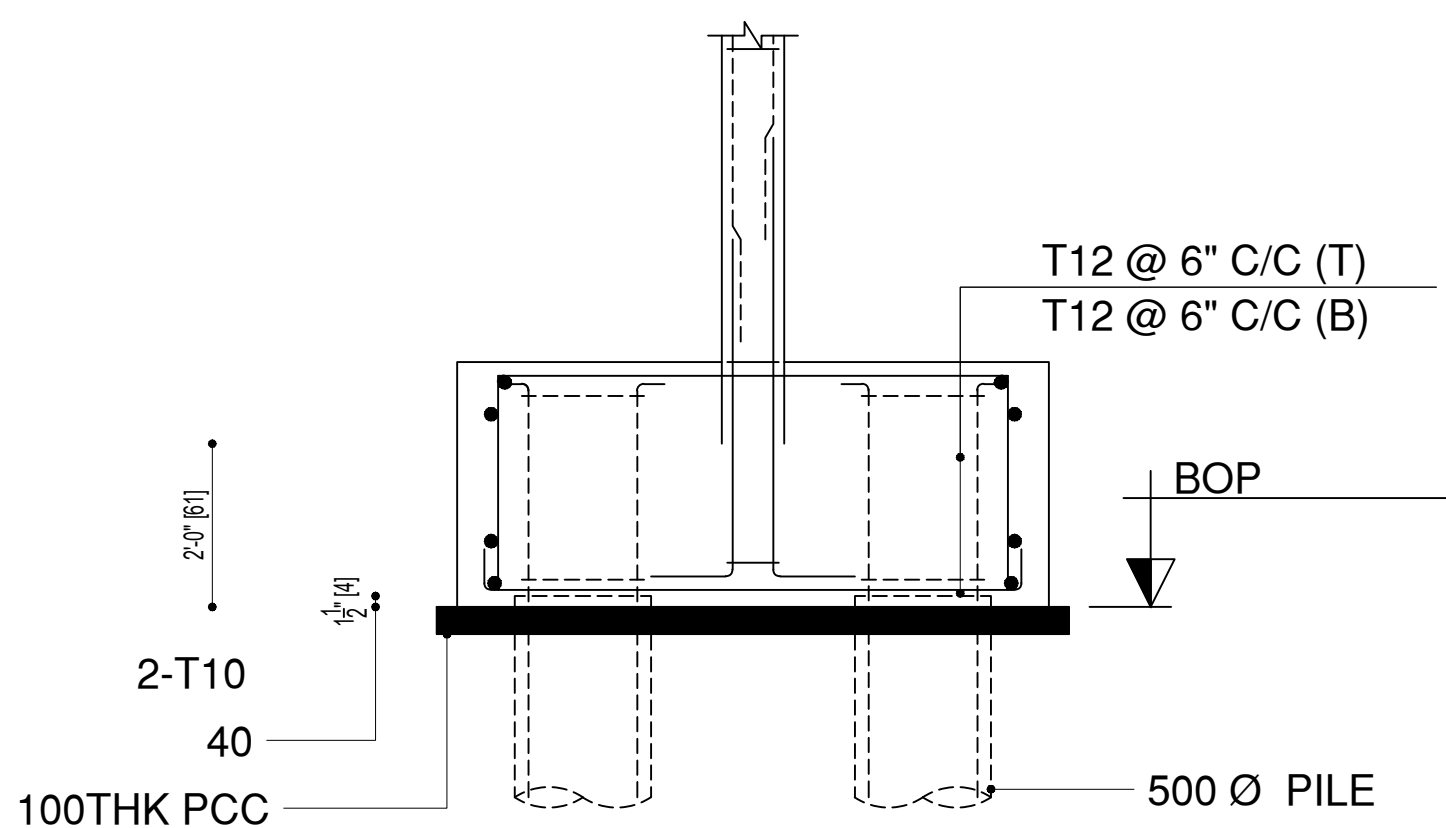
SECTION - S1 - S1
