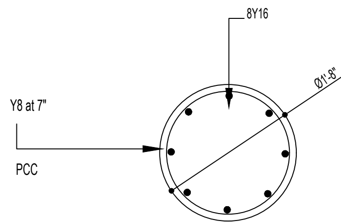
CROSS - SECTION OF PILE
