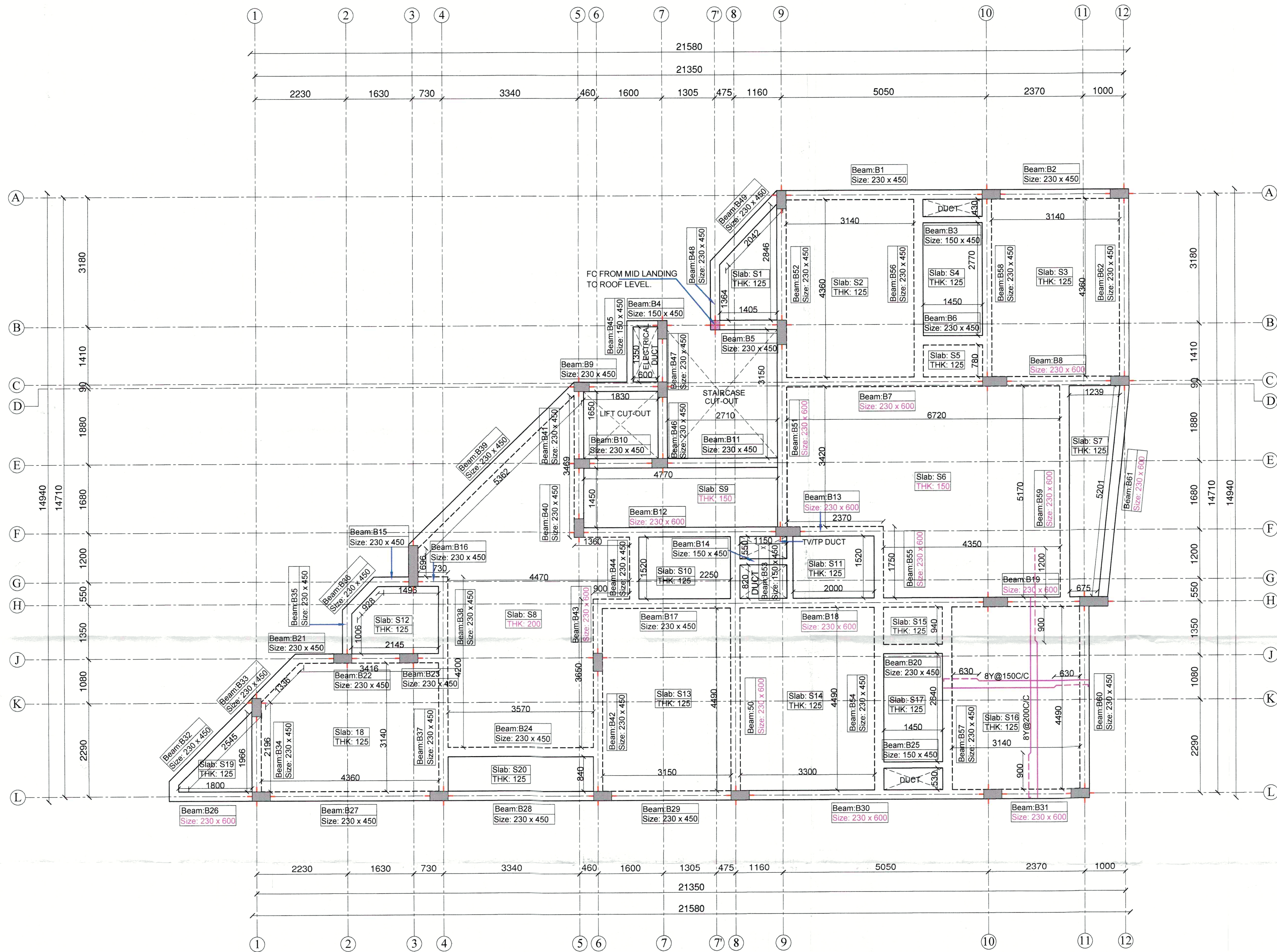
TERRACE FLOOR ROOF BEAM LAYOUT
