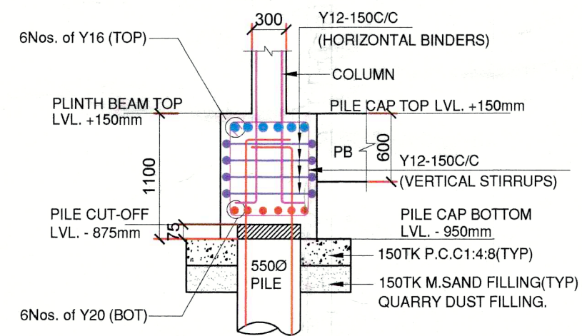
SECTION 1-1
