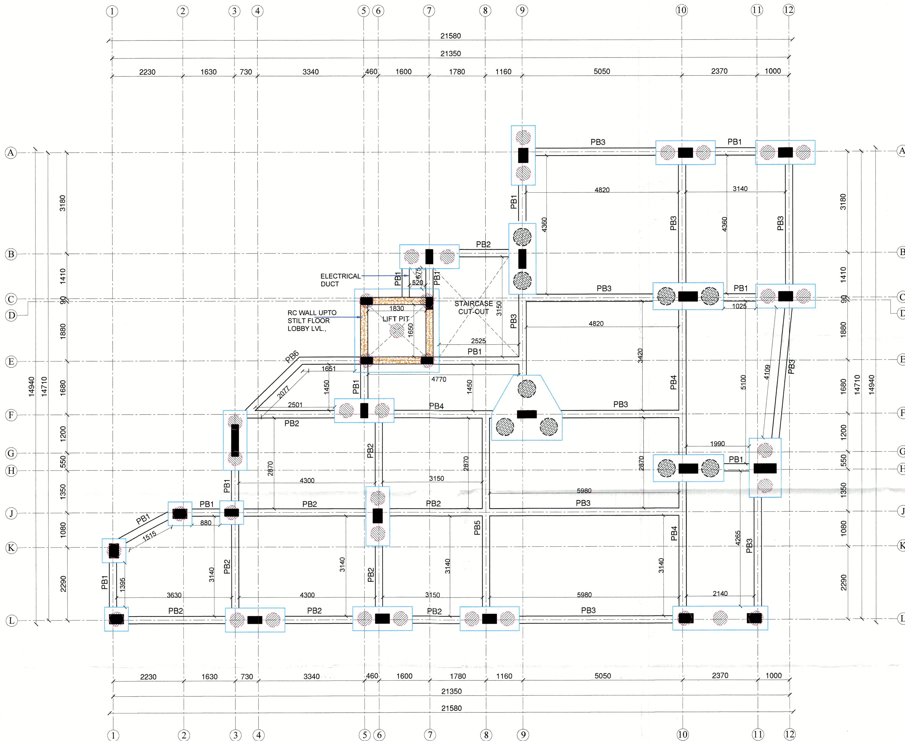
PLINTH BEAM LAYOUT
