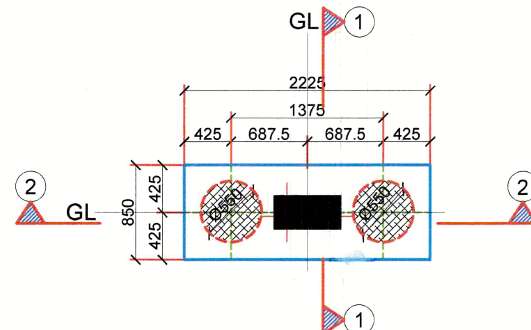
TYPICAL PLAN PILE CAP-P4- 550Ø PILE
