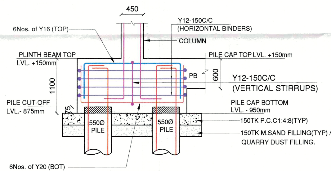
SECTION 2-2
