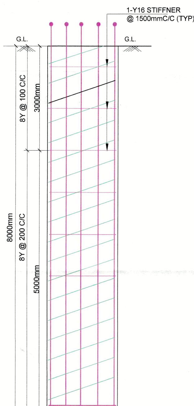
TYPICAL SECTION OF PILE (BORED CAST IN-SITU PILE)
