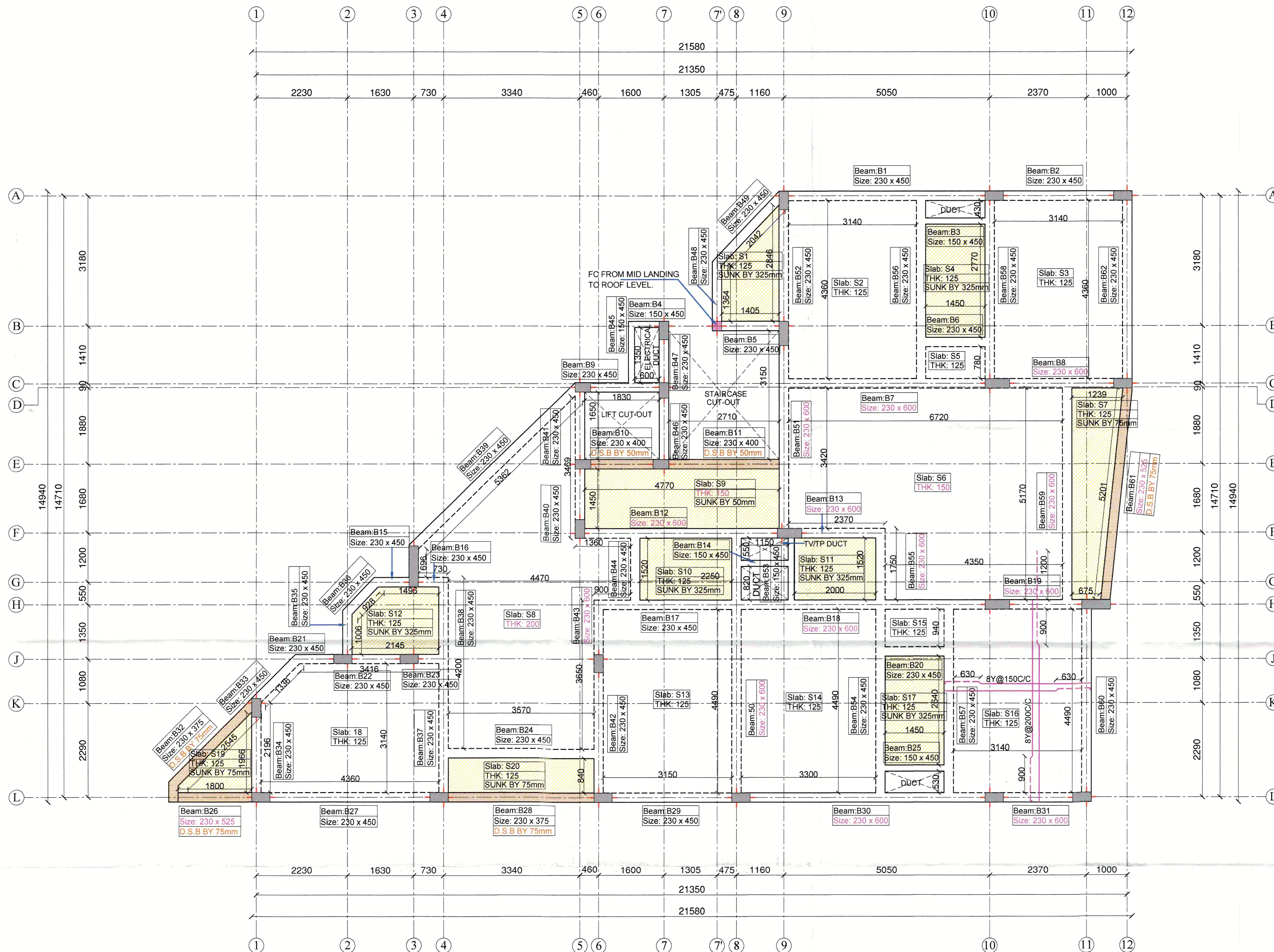
TYPICAL FLOOR ROOF BEAM LAYOUT ( FIRST, SECOND, THIRD AND FOURTH )
