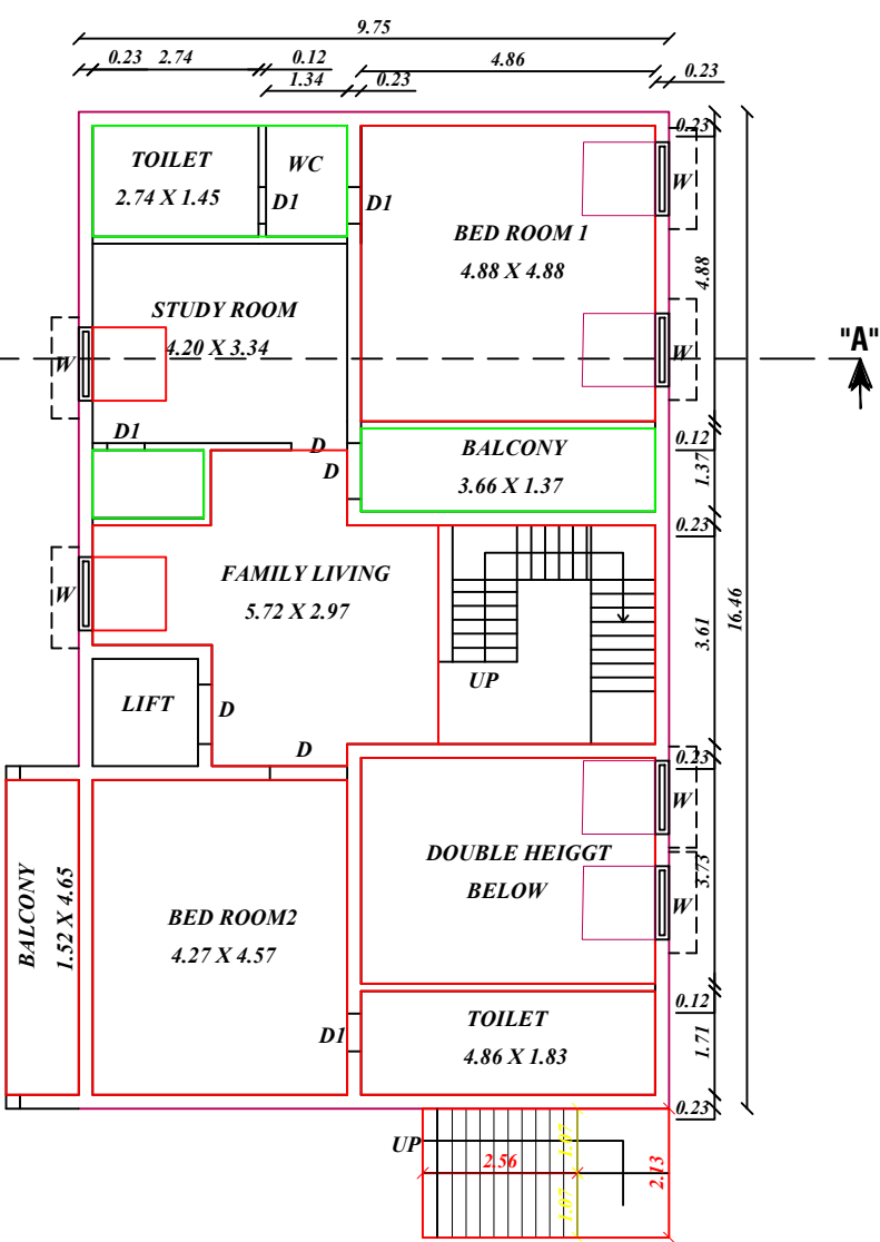
FLOOR - TERRACE
