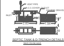
SEPTIC TANK & D-TRENCH DETAILS NOT TO SCALE
