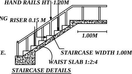
HAND RAILS HT-1.20M
