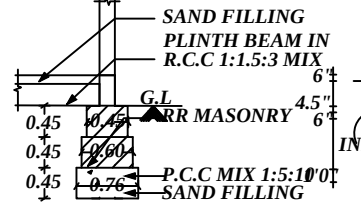
RR MASONRY DETAILS
