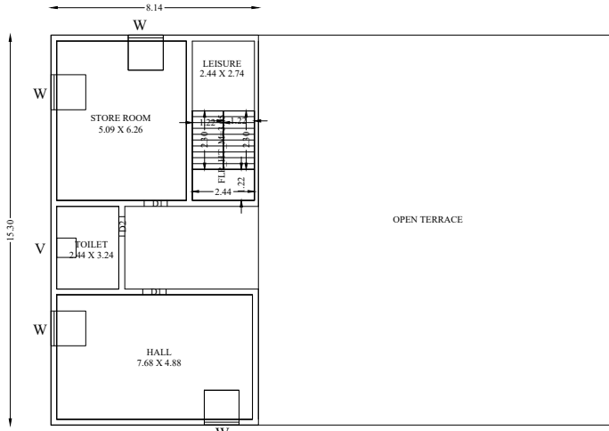
PROPOSED SECOND FLOOR PLAN
