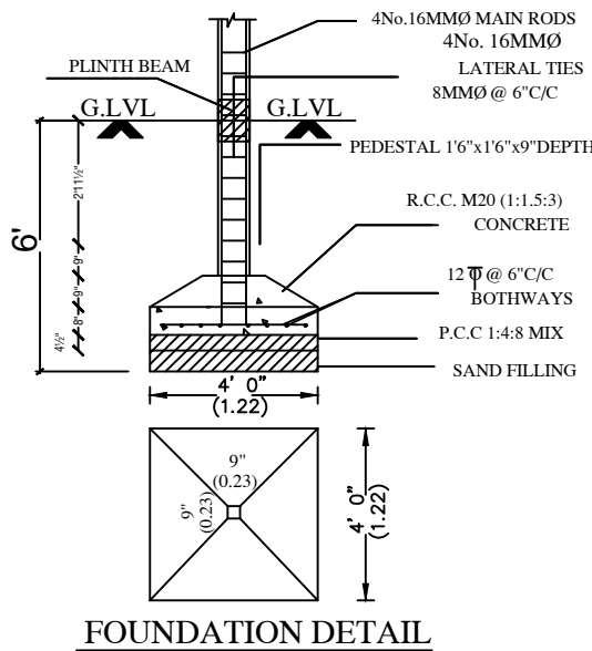
FOUNDATION DETAIL
