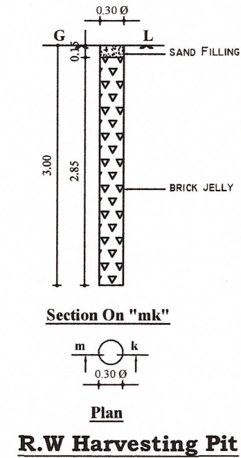
R.W Harvesting Pit
