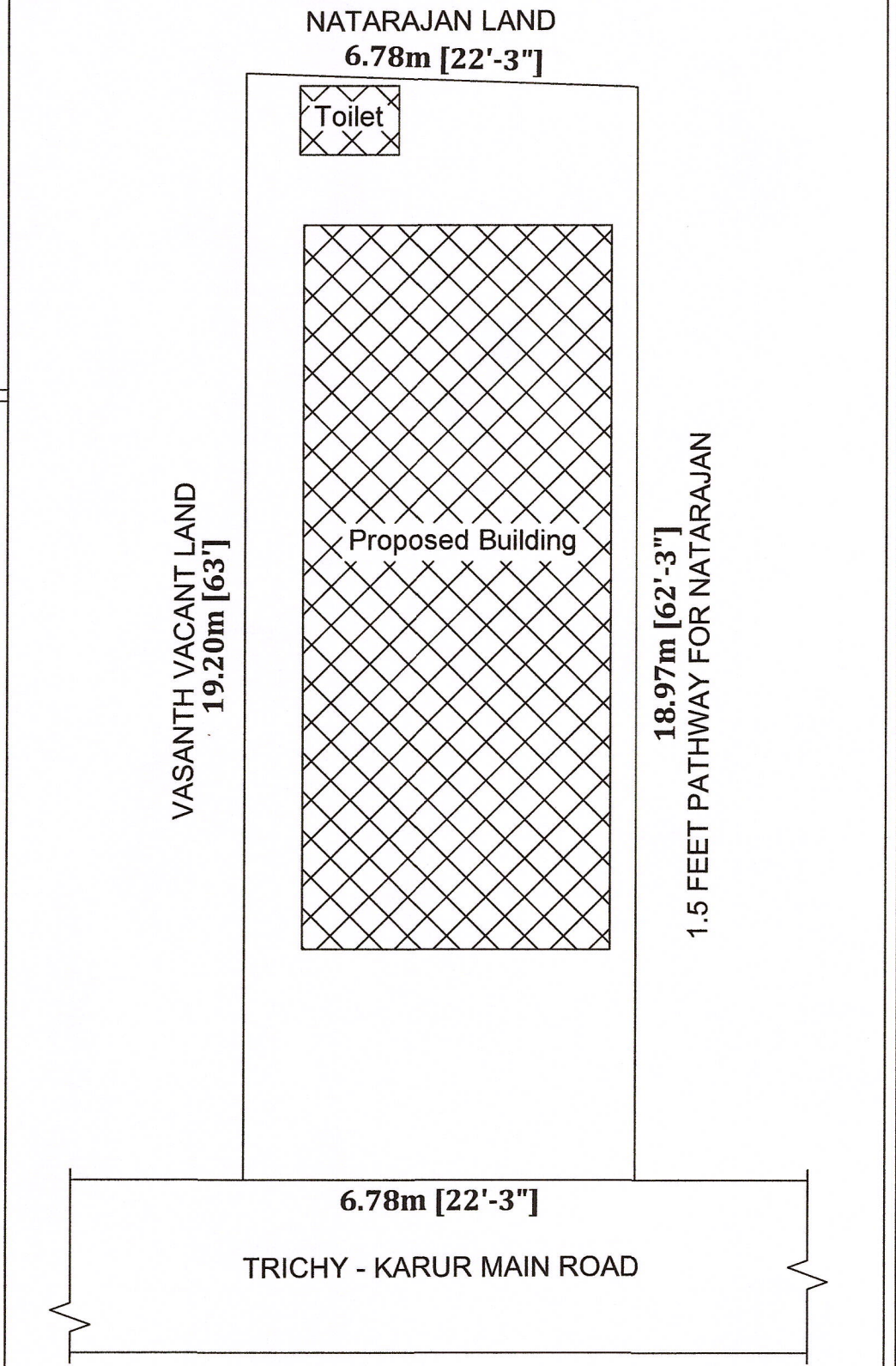
SITE PLAN
