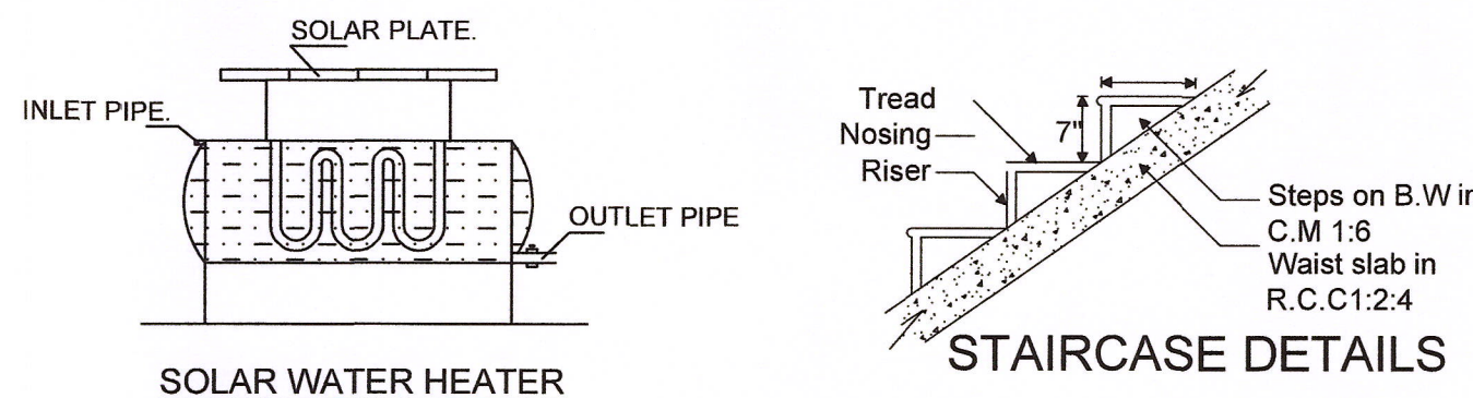
SOLAR WATER HEATER STAIRCASE DETAILS
