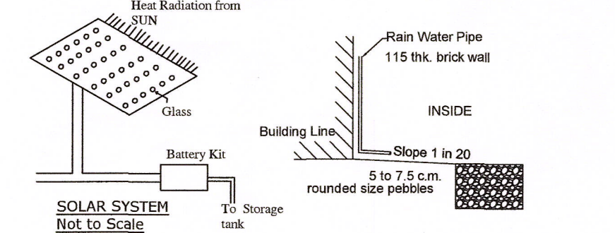
SOLAR SYSTEM Not to Scale
