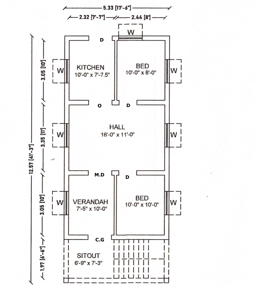
FLOOR PLAN - GROUND [PROPOSED]
