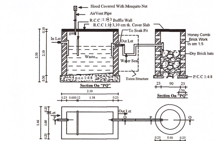
Septic Tank Details Soak Pit Details (SCALE-1:50)
