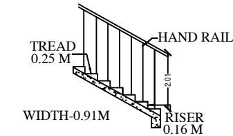
STAIRCASE DETAILS
