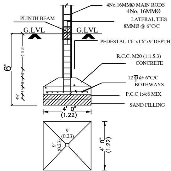
FOUNDATION DETAIL
