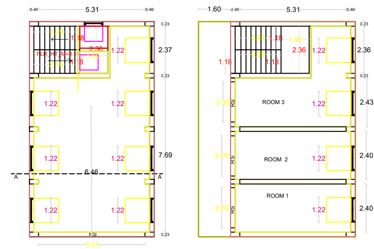
FLOOR PLAN 0
