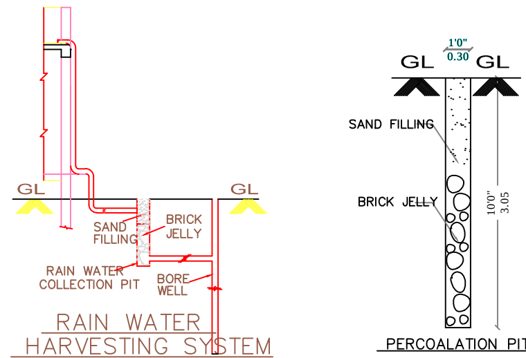
PERCOLATION PIT
