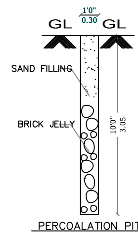
PERCOLATION PIT
