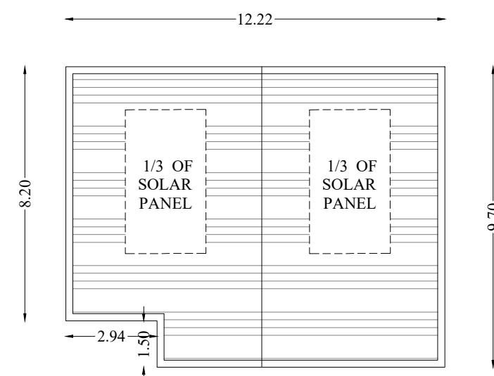
TERRACE FLOOR
