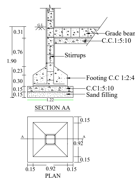
FOUNDATION DETAILS
