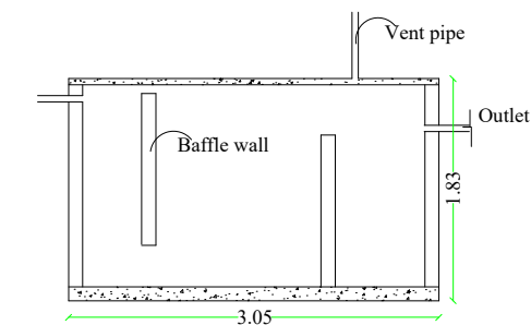
SEPTIC TANK DETAILS Size: 3.05 x 1.83 SCALE 1:100
