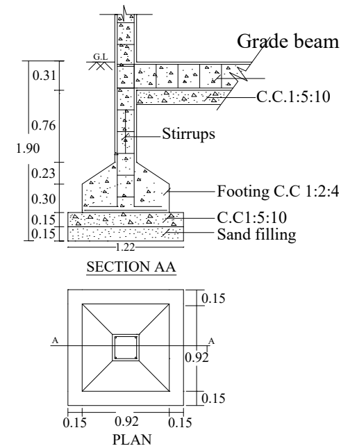
FOUNDATION DETAILS
