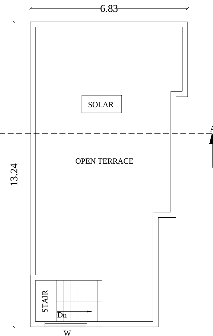
TERRACE FLOOR
