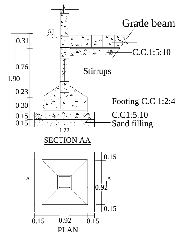
FOUNDATION DETAILS
