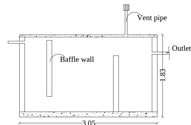
SEPTIC TANK DETAILS Size: 3.05 x 1.83 SCALE 1:100
