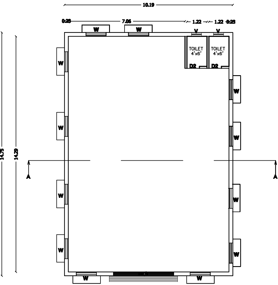
PLAN
