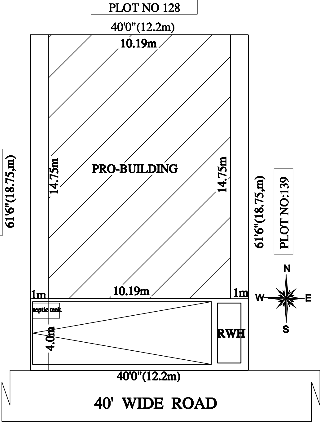
SITE PLAN
