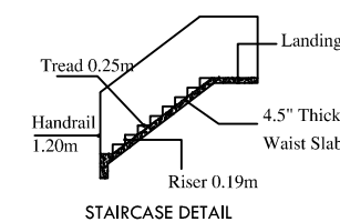
STAIRCASE DETAIL
