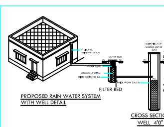
ENCLOSED RAIN WATER SYSTEM WITH WELL DETAIL
