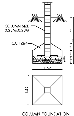
COLUMN FOUNDATION
