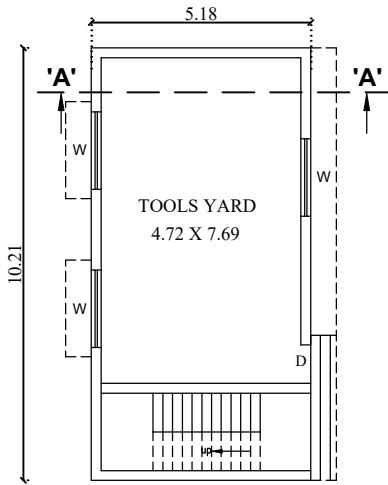
GROUND FLOOR PLAN BLOCK No. 1
