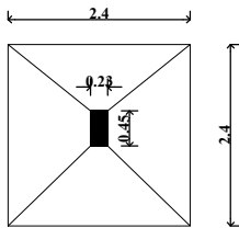
PLAN OF COLUMN FOUNDATION
