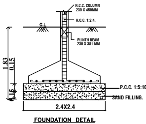
FOUNDATION DETAIL
