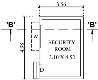
GROUND FLOOR PLAN BLOCK No.2
