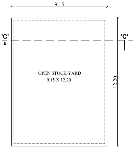
PLAN BLOCK No. 4
