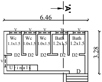
GROUND FLOOR PLAN BLOCK No.3
