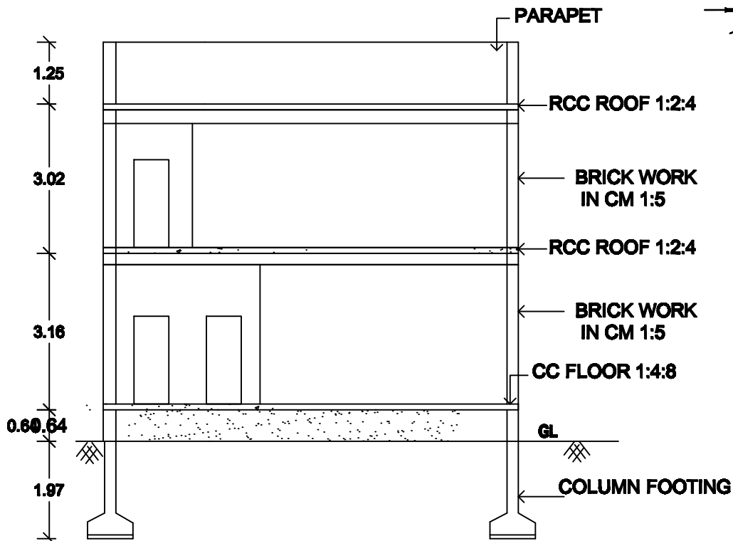
SECTION AB
