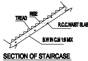
SECTION OF STAIRCASE
