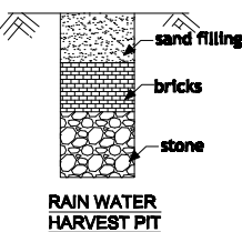
RAIN WATER HARVEST PIT
