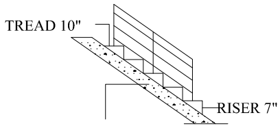
STAIRCASE DETAILS [N.T.S.]
