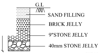
RAIN WATER HARVESTING RECHARGE PIT
