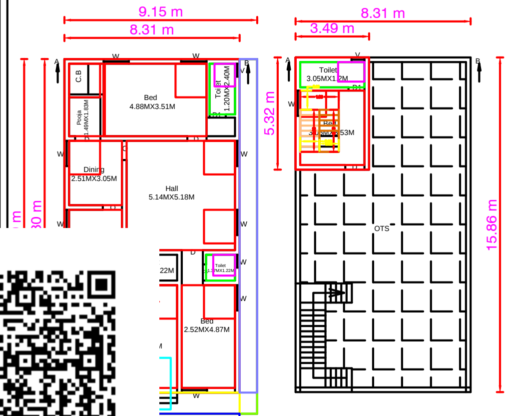
FIRST FLOOR(Pro.)
