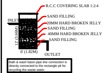
Section - 'CD' Not To Scale
