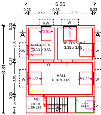
GROUND FLOOR PLAN (NORTH FACING)
