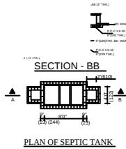
PLAN OF SEPTIC TANK
