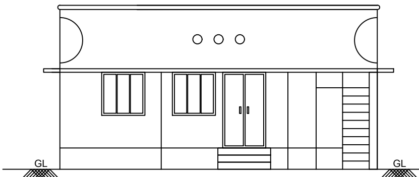
FRONT ELEVATION
