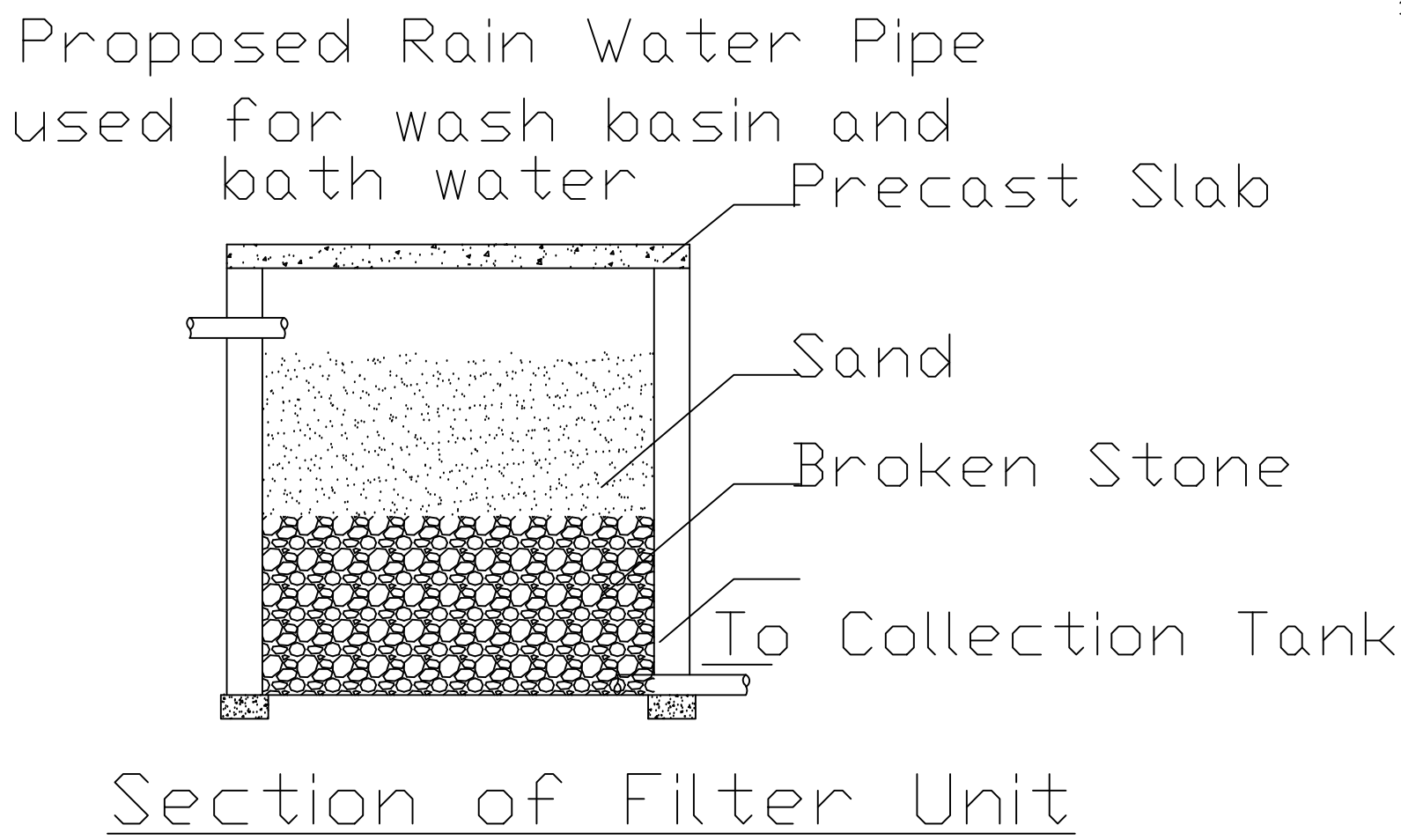
Section of Filter Unit
