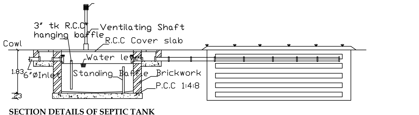
SECTION DETAILS OF SEPTIC TANK
