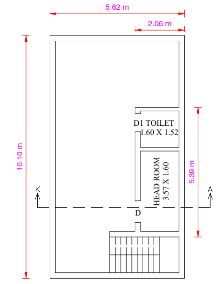
FIRST & TERRACE FLOOR PLAN
