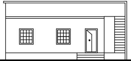
FRONT ELEVATION
