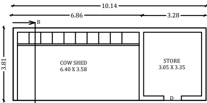
COW SHED PLAN
