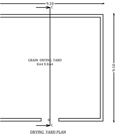
DRYING YARD PLAN
