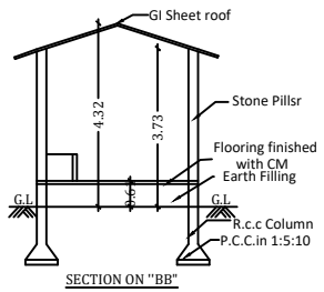
SECTION ON "BB"
