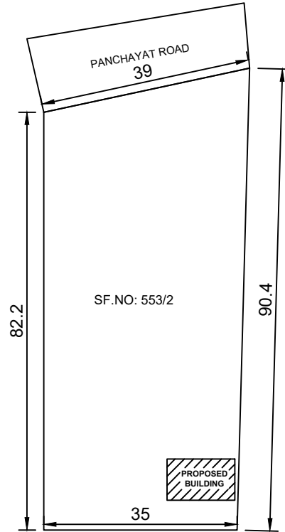
SITE PLAN SHOWN IN SHEET 2
