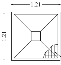
PLAN MAT USING 10 # BOTH SIDES
