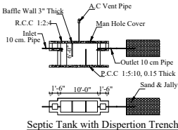
Septic Tank with Dispersion Trench
