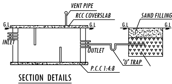
SECTION DETAILS
