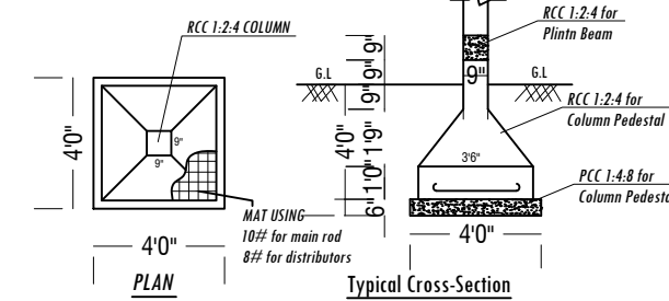
FOOTING DETAILS
