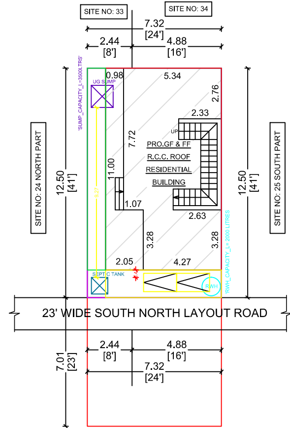
SITE PLAN
