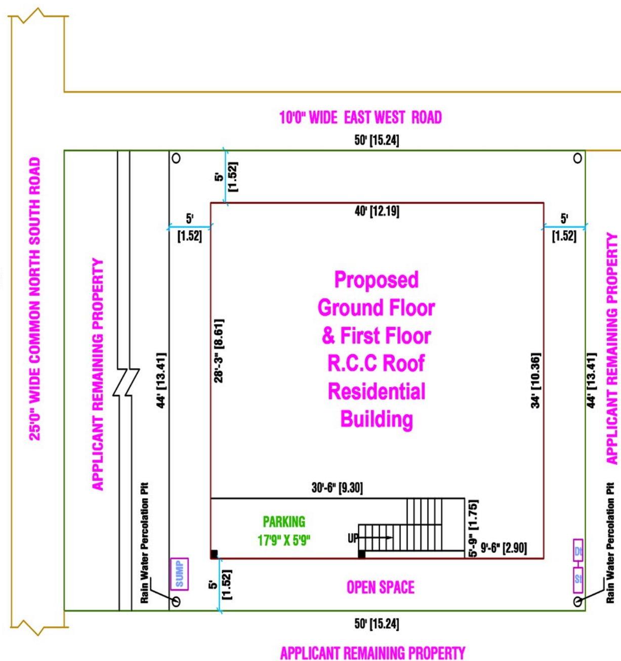
SITE PLAN SCALE 1" : 8' 0"
