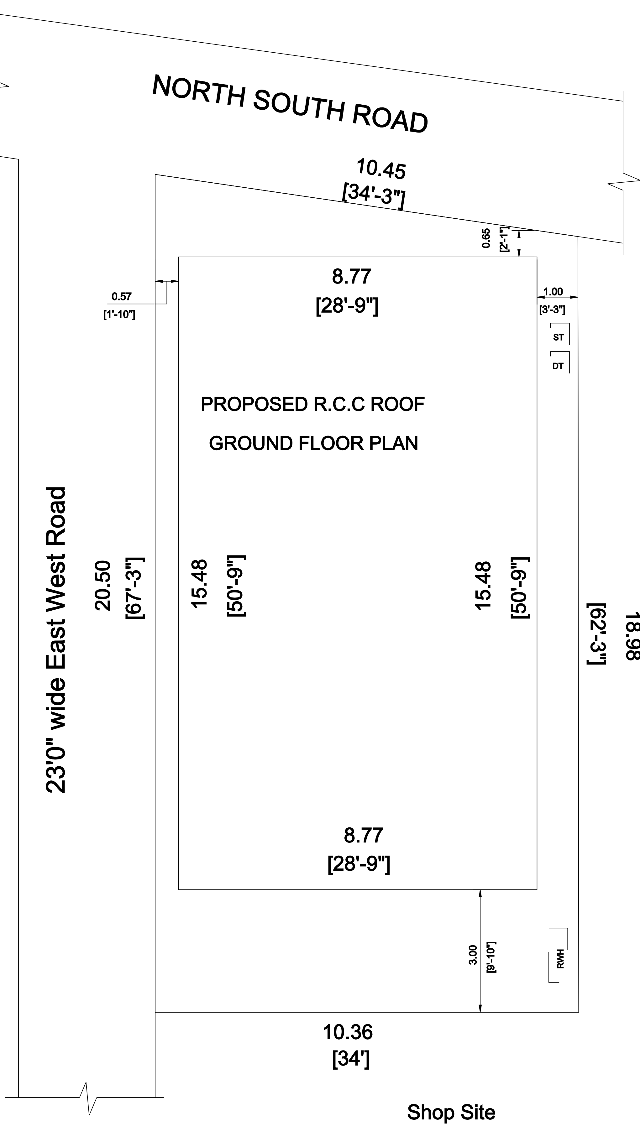
SITE PLAN
