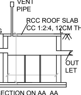
SECTION ON AA AA
