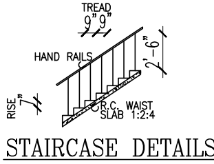
STAIRCASE DETAILS
