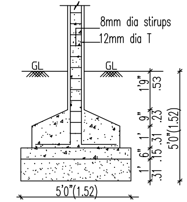
COLUMN FOUNDATION DETAIL
