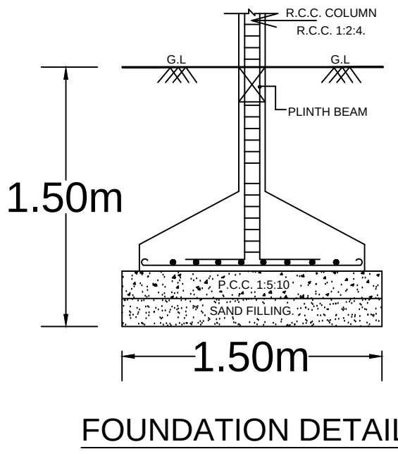
FOUNDATION DETAIL
