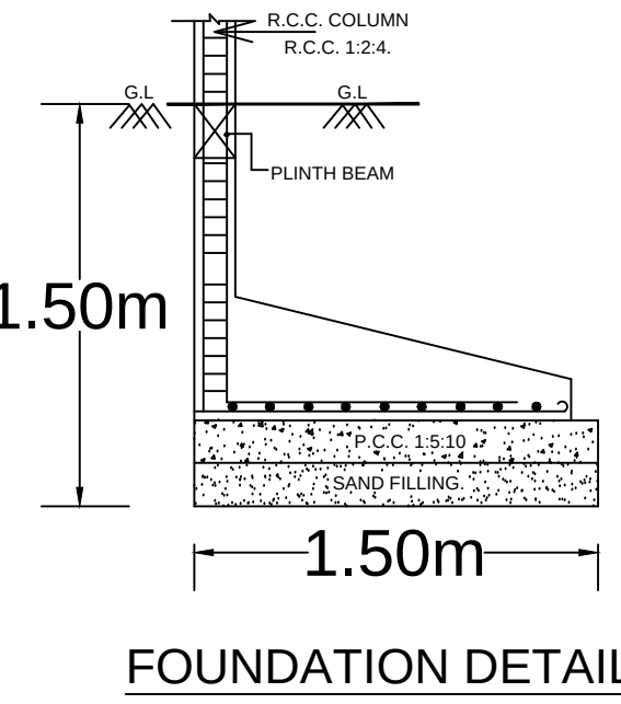
FOUNDATION DETAIL
