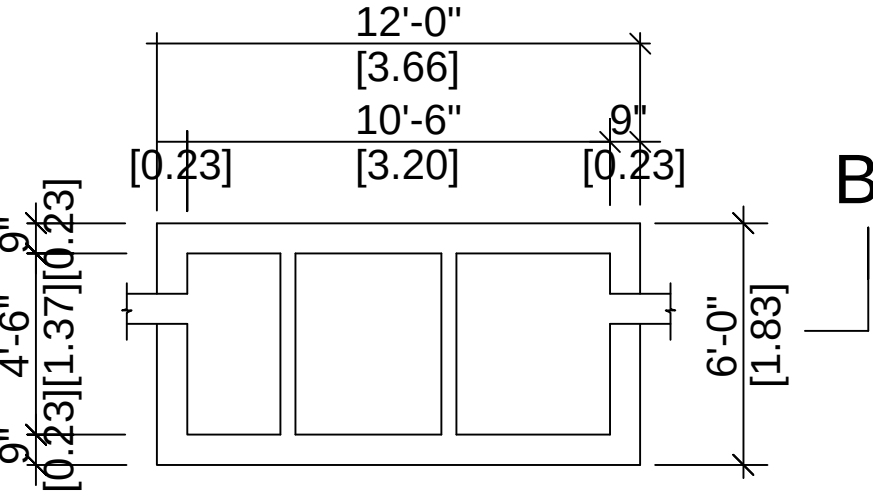
PLAN SEPTIC TANK DETAILS
