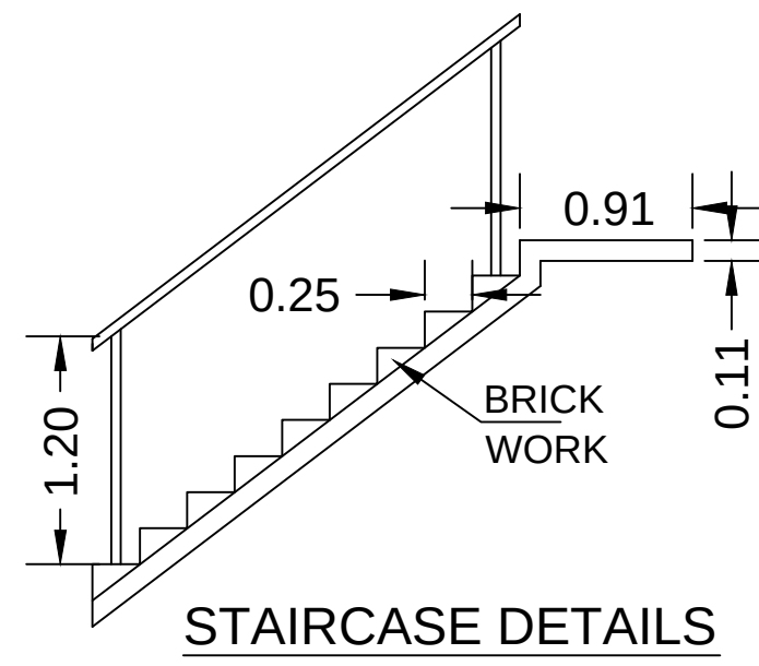
STAIRCASE DETAILS
