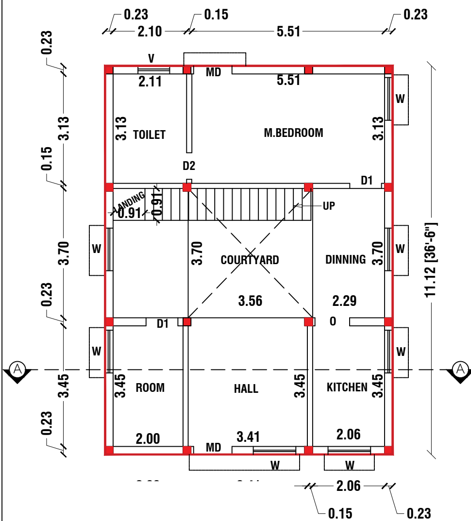
PLAN
